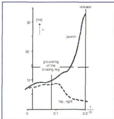
Figure 2: Velocity-time curves of the movement of the Javelin and the hips (Uwe Hohn: 104.80m)
