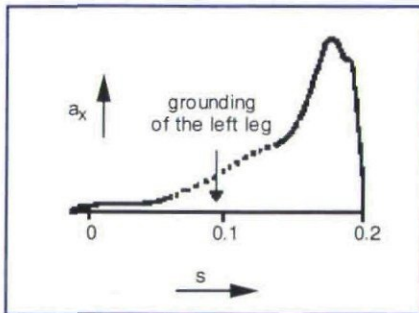
Figure 7b: Acceleration curve in the case of a bent throwing arm
