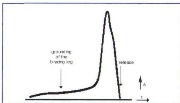
Figure 4: Ideal acceleration curve
