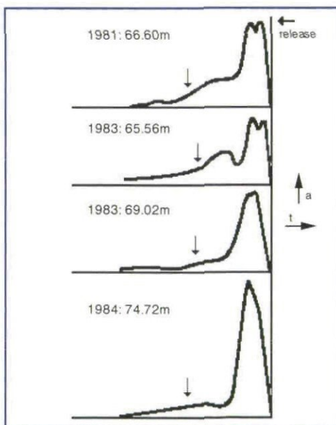
Figure 6: Acceleration curves of throws by Petra Felke. (The arrows indicate the grounding of the bracing leg)
