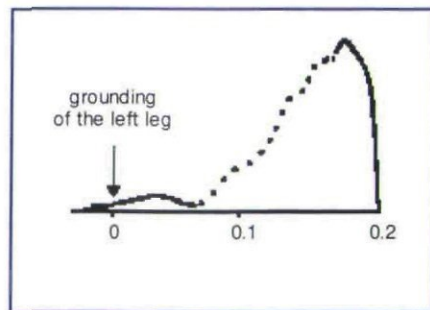
Figure 8b: Acceleration curve in the case of a bent bracing leg
